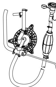
OG.426.00 BOOSTER AND FILLING PUMP
